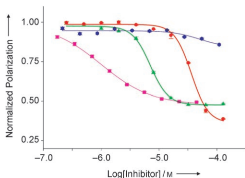
Figure 4. Titration curves for compounds 1 (red), 5 (blue), 6 (green), and control peptide SRC-1 NR II (pink).
